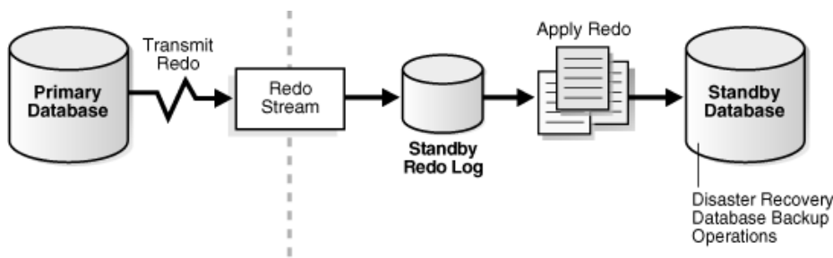
Figure 3: Typical Oracle Data Guard Configuration
